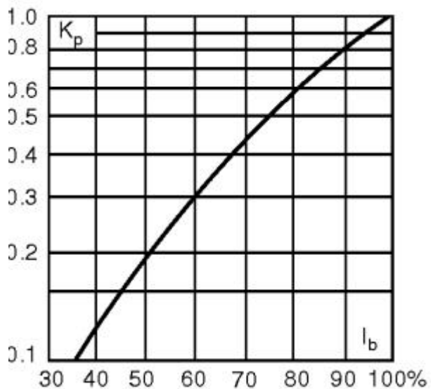
Power Losses
