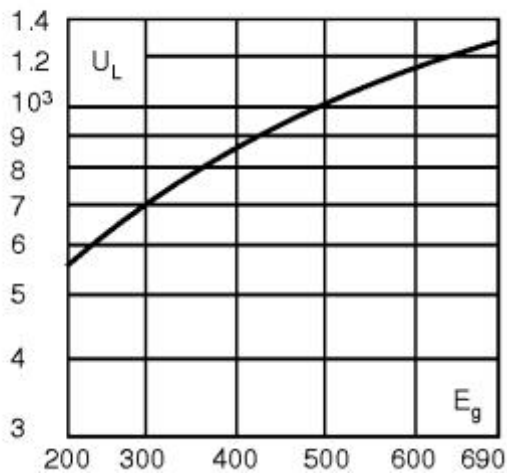
Arc Voltage
