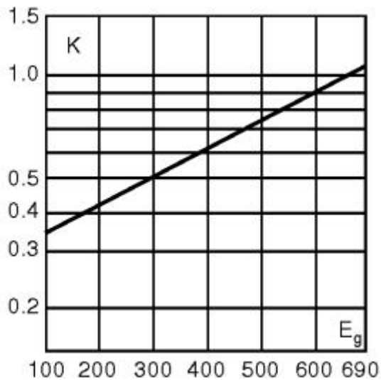
Total Clearing I2t
